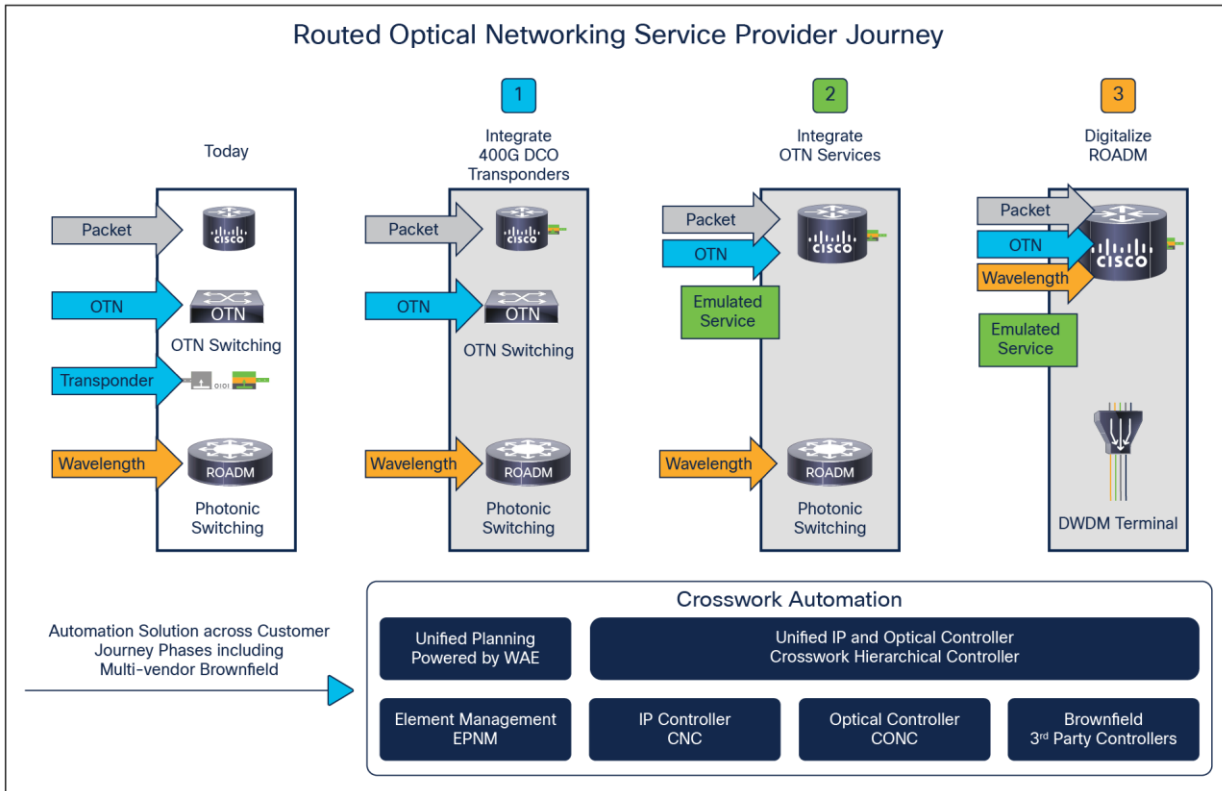
Figure 4. Service provider journey through Routed Optical Networking deployment phases
