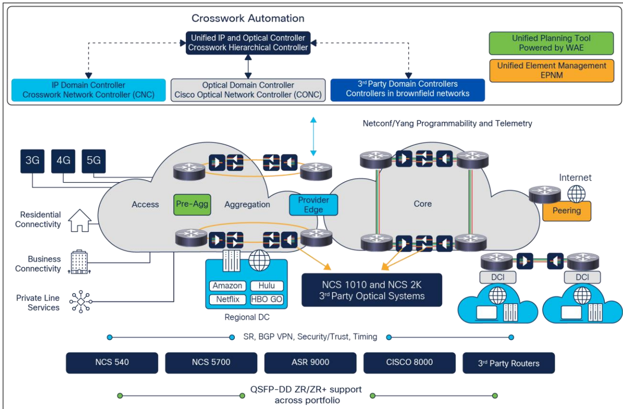
Figure 3. Cisco's Routed Optical Networking portfolio
